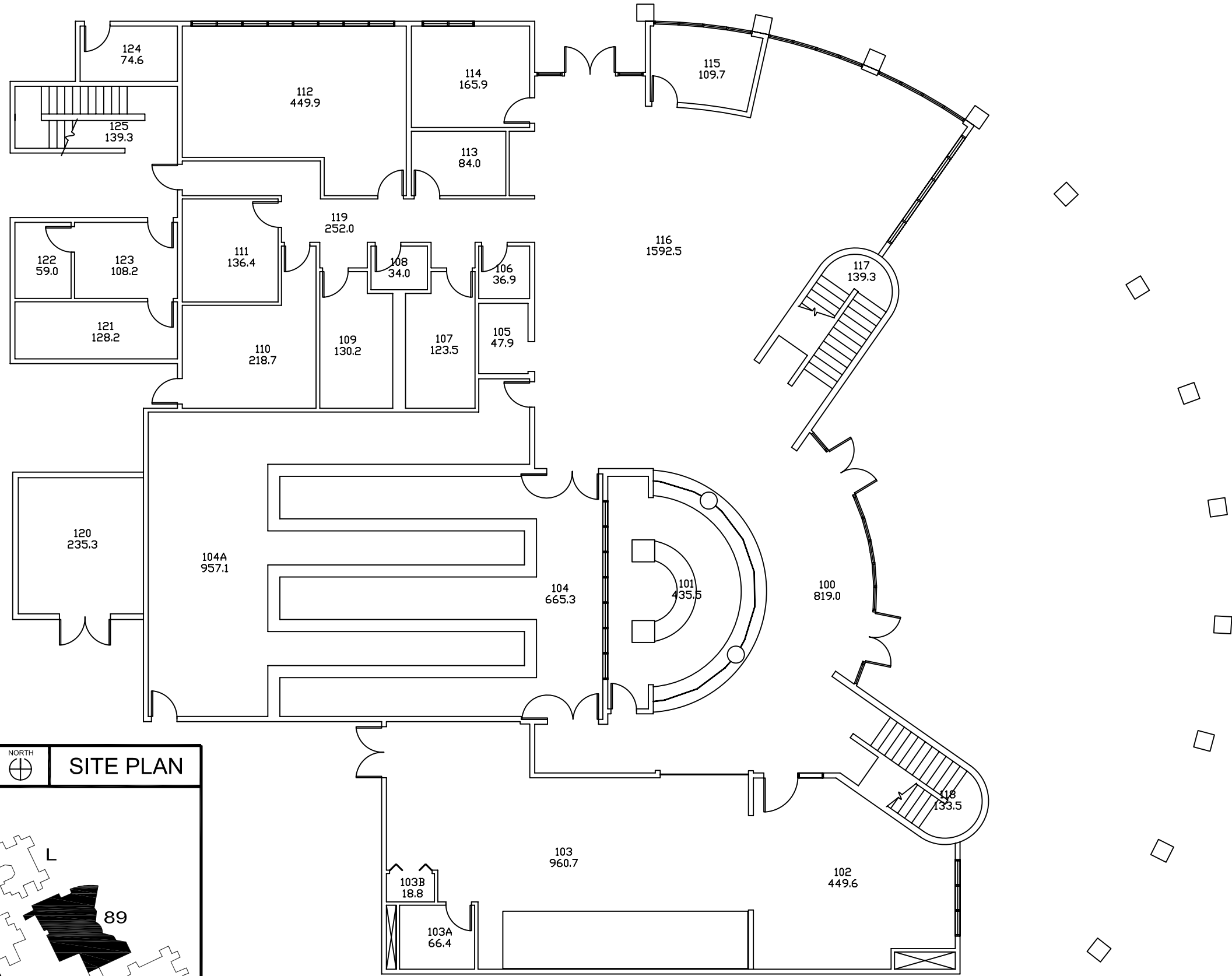
FIRST FLOOR SCALE: NOT TO SCALE
